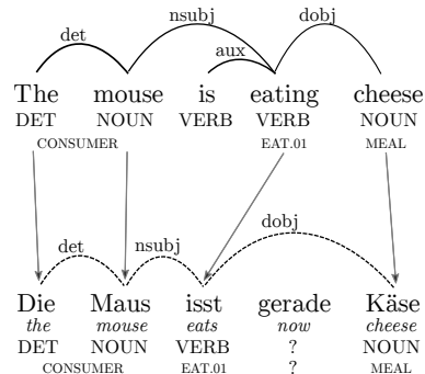
Figure 1: An English sentence with syntactic and semantic annotations predicted by a parser, and a German translation. These annotations are transferred onto aligned German words, thus automatically labeling the German sentence (with exception of the unaligned German word gerade ).
